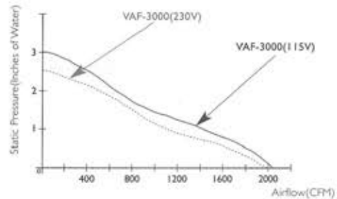
PERFORMANCE CURVES
